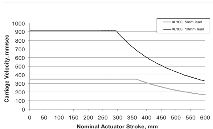
XL100 - Maximum Permissible Carriage Velocity
