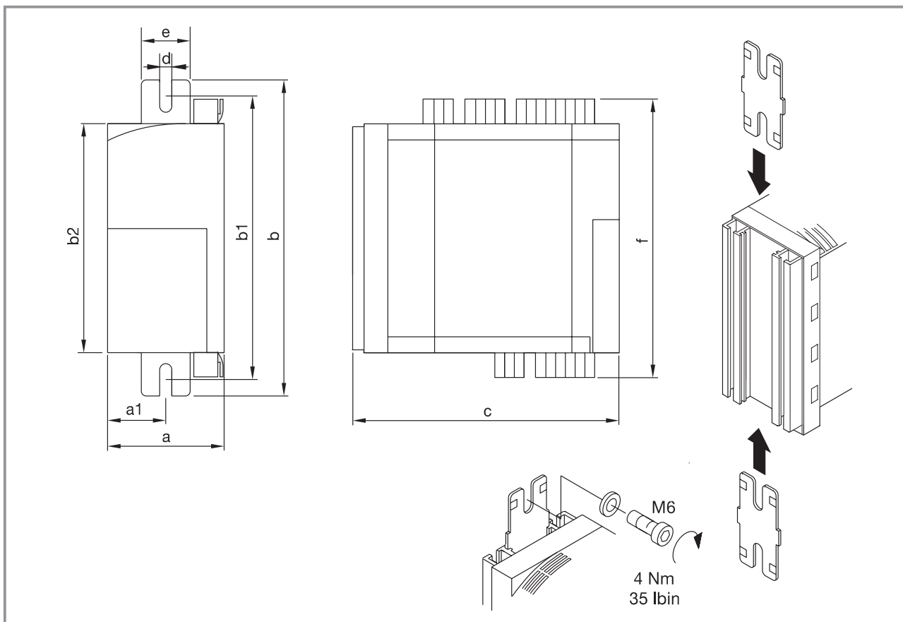
Dimensions [mm]
