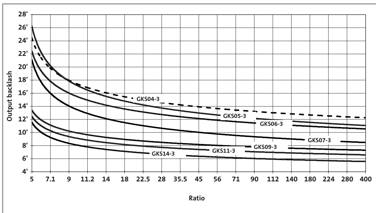
Helical-bevel gearboxes GKS□□-3
