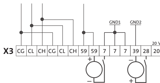
Supply for function module and controller inhibit (CINH) via external voltage source
