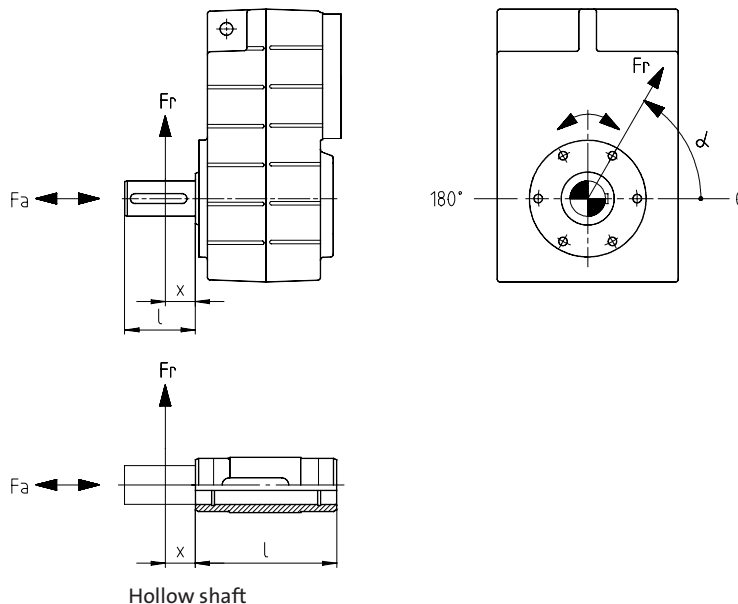
Hollow shaft
