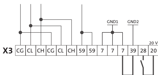
Supply for controller inhibit (CINH) via internal voltage source (X3/20)
