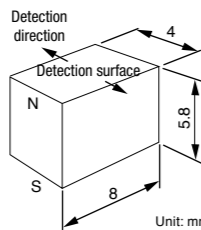
Magnet PG-9104 singly PG-9104
