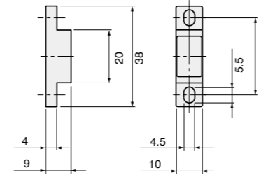
SET-P15 Magnet PG-104(PG-10)
