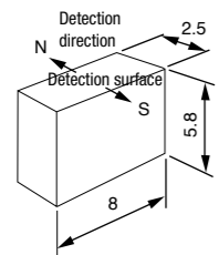
Magnet PG-9010 (for SET-P15/-P16) singly
