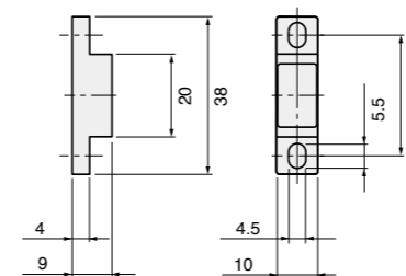
SET-P16 Magnet PG-104
