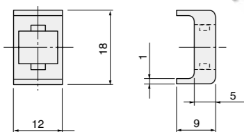
Magnet PG-9010 (for SET-P15/-P16) singly
